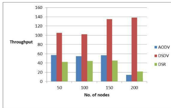
Figure 2: Throughput
