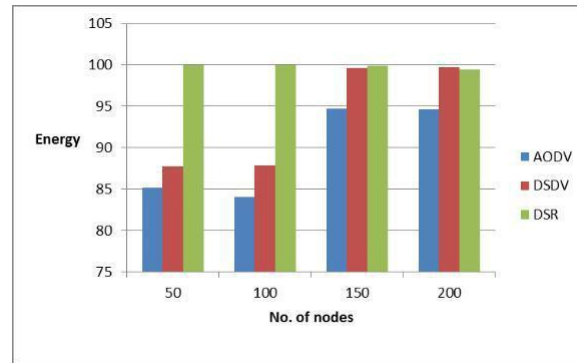
Figure 4: Residual Energy
